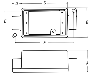
Fig. C Thru-Feed
